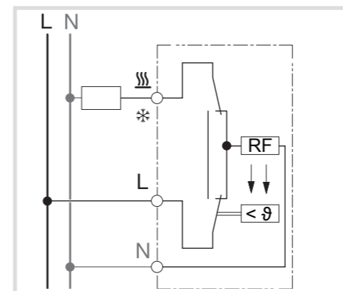
Figure 4: Electrical connection
