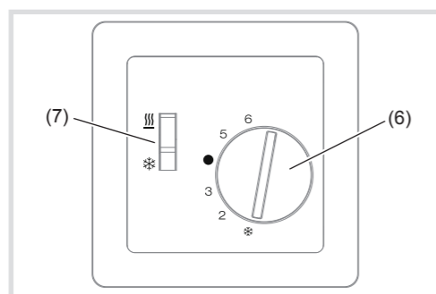
Figure 2: Operating elements
