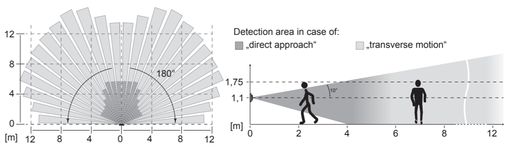
Fig 6: Detection area of the radio motion detector 1,1 m
