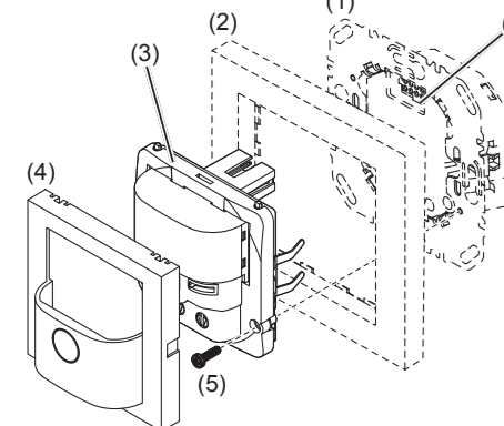
Figure 1: Design of the device
