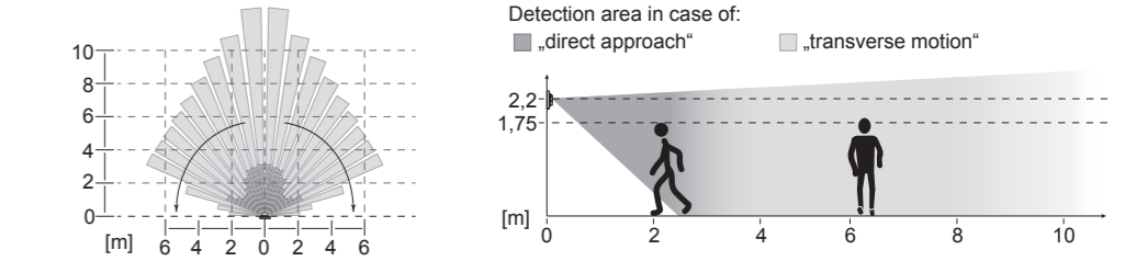
Fig 7: Detection area of the radio motion detector 2,2 m
