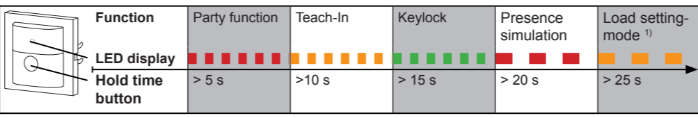
Fig. 3: Selection of the special functions and LED display
