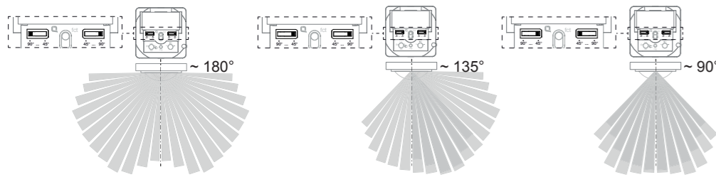
Fig. 8: Setting the detection angle
