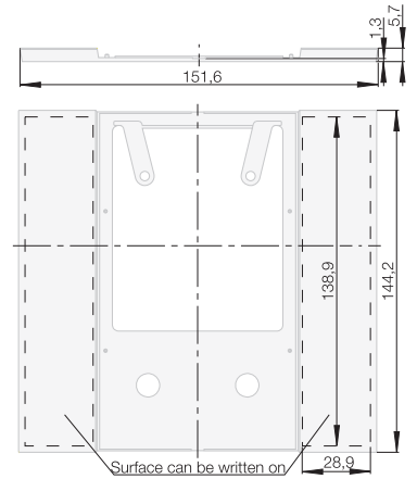
Labelling field for B,I,Q push-button 5gang
