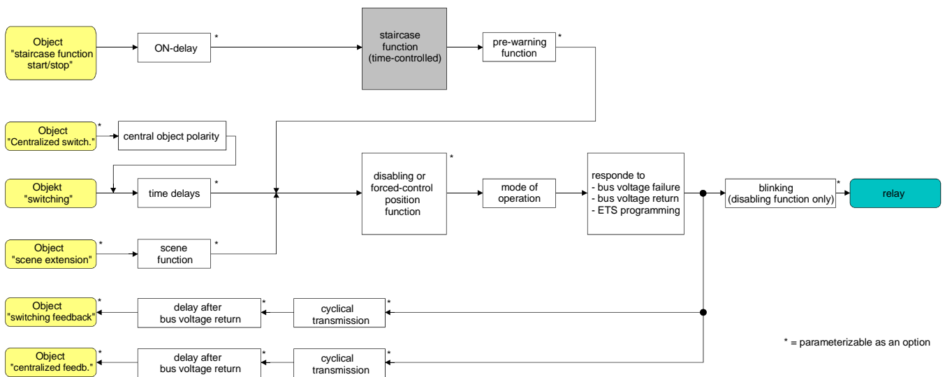
Fig. 14: Functional diagram of the staircase function
