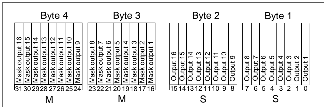
Fig. 9: Structure of the centralized feedback object
