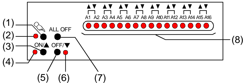
Fig. 6: Controls and indicators for manual control for switching/shutter actuator 8/16fold
