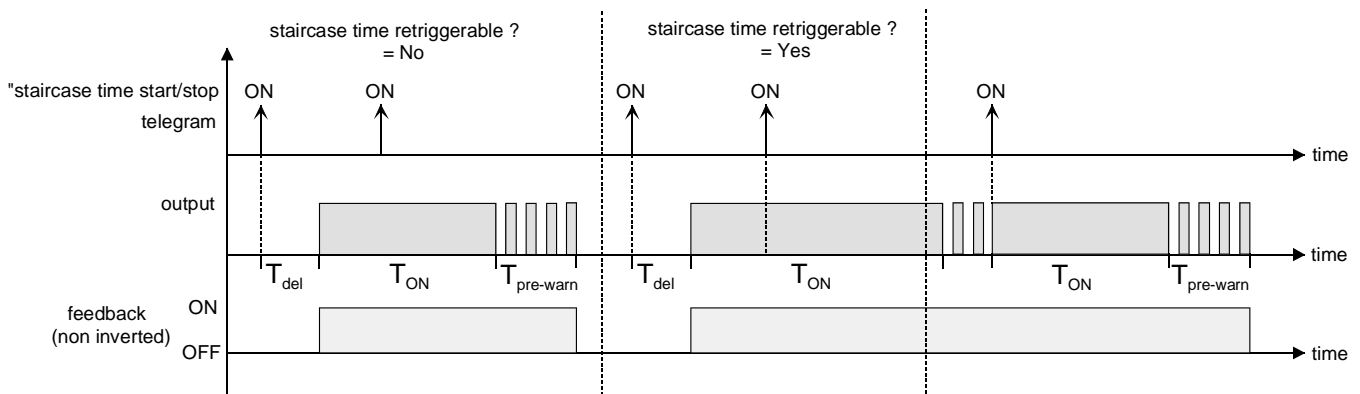
Fig. 15: Switch-on behaviour of the staircase function
