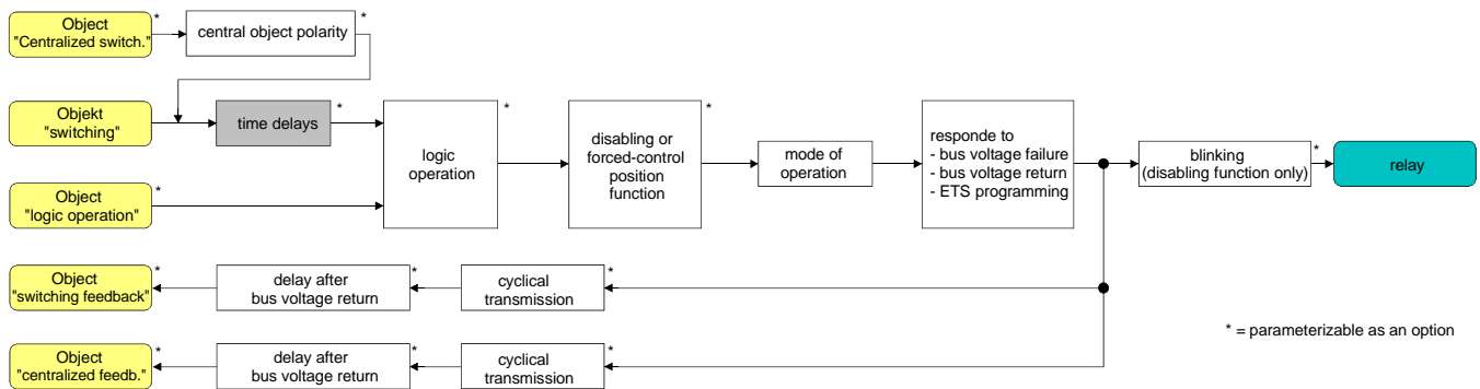
Fig.13: Functional diagram of the time delays
