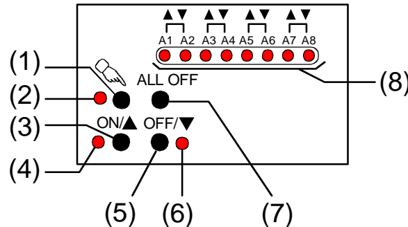
Fig. 5: Controls and indicators for manual control for switching/shutter actuator 4/8fold
