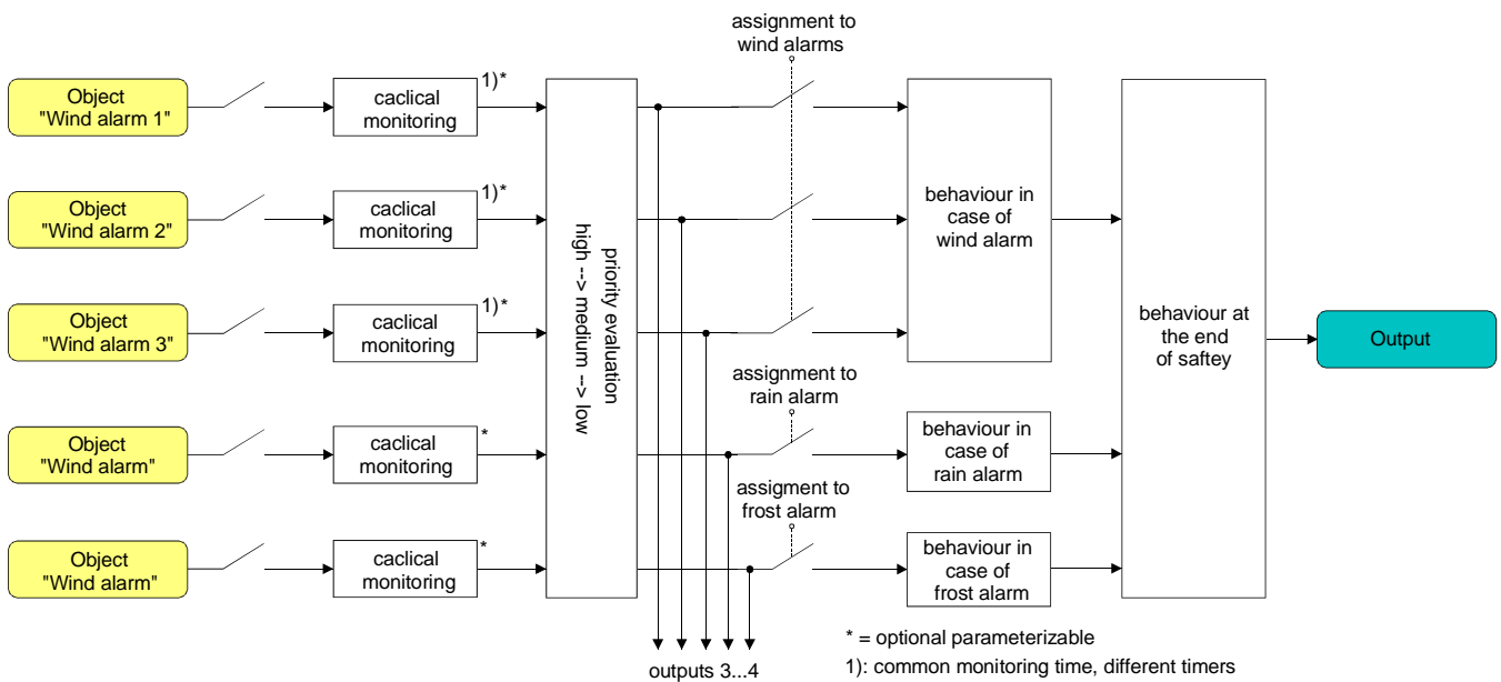
Fig. 30: Function diagram of channel-oriented safety functions
