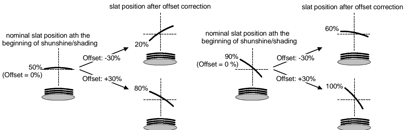
Fig. 34: Functional principle of slat offset (example showing slat type 1 / slat type 2 identical)
