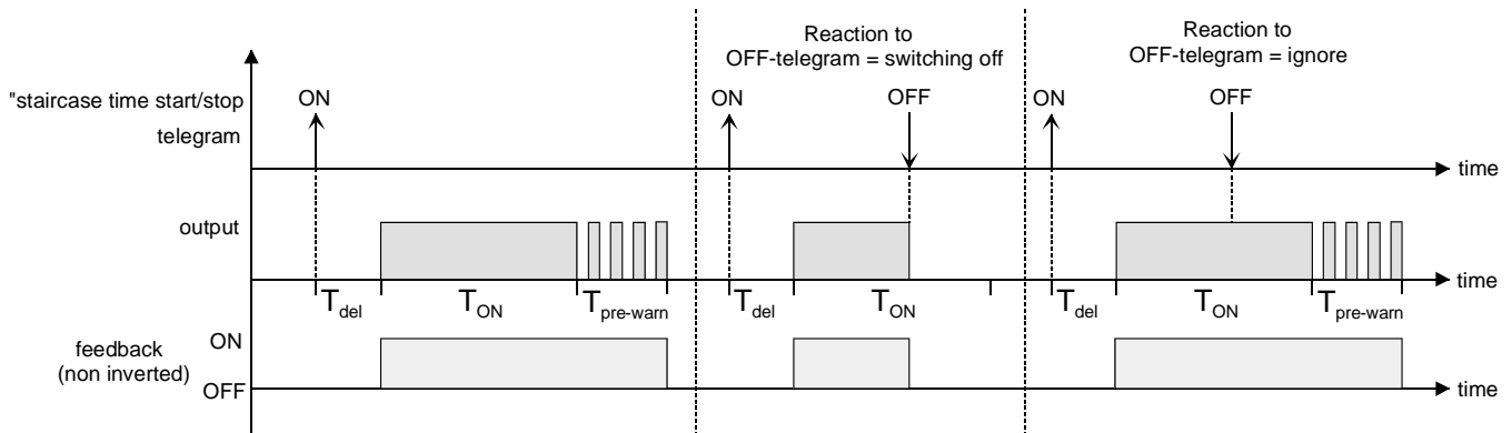
Fig. 16: Switch-off behaviour of the staircase function
