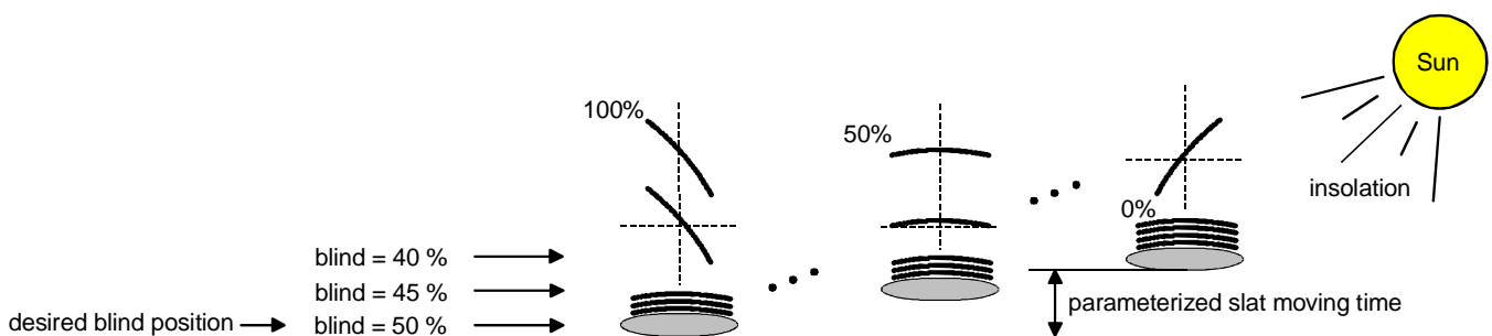
Fig. 27: Example of slat positioning affecting the position of the blind (typical of slat type 1; analogous reaction for type 2)
