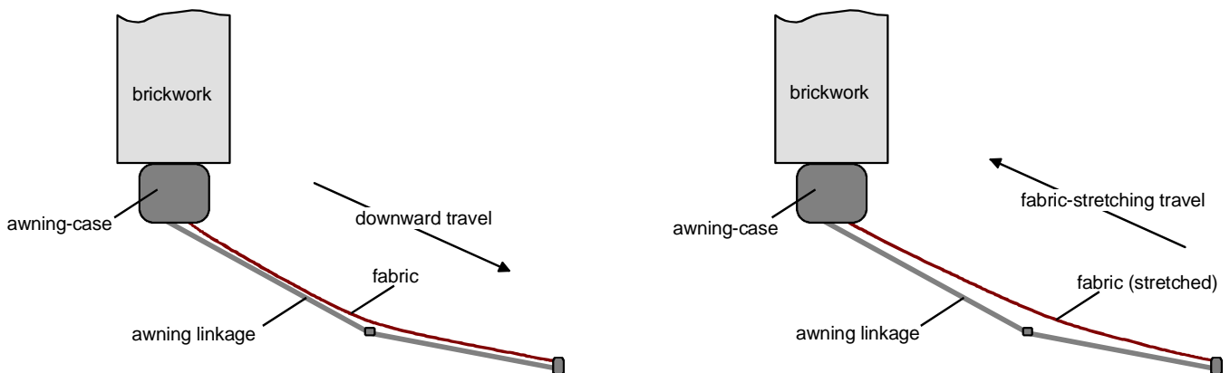
Fig. 40: Fabric-stretching in an awning
