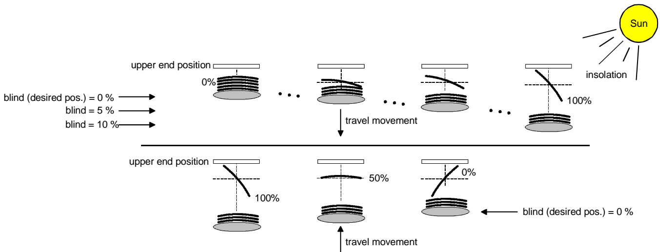
Fig. 28: Example of slat positioning with the blind in upper end position (typical of slat type 1)
