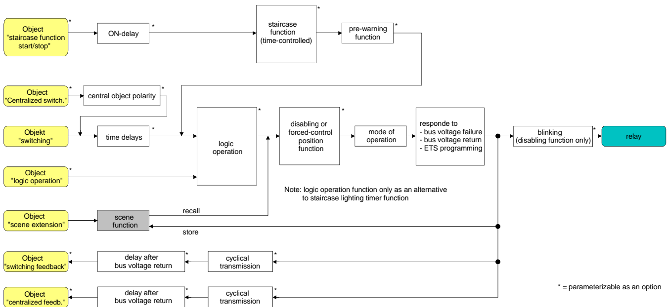
Fig. 18: Functional diagram of the scene function
