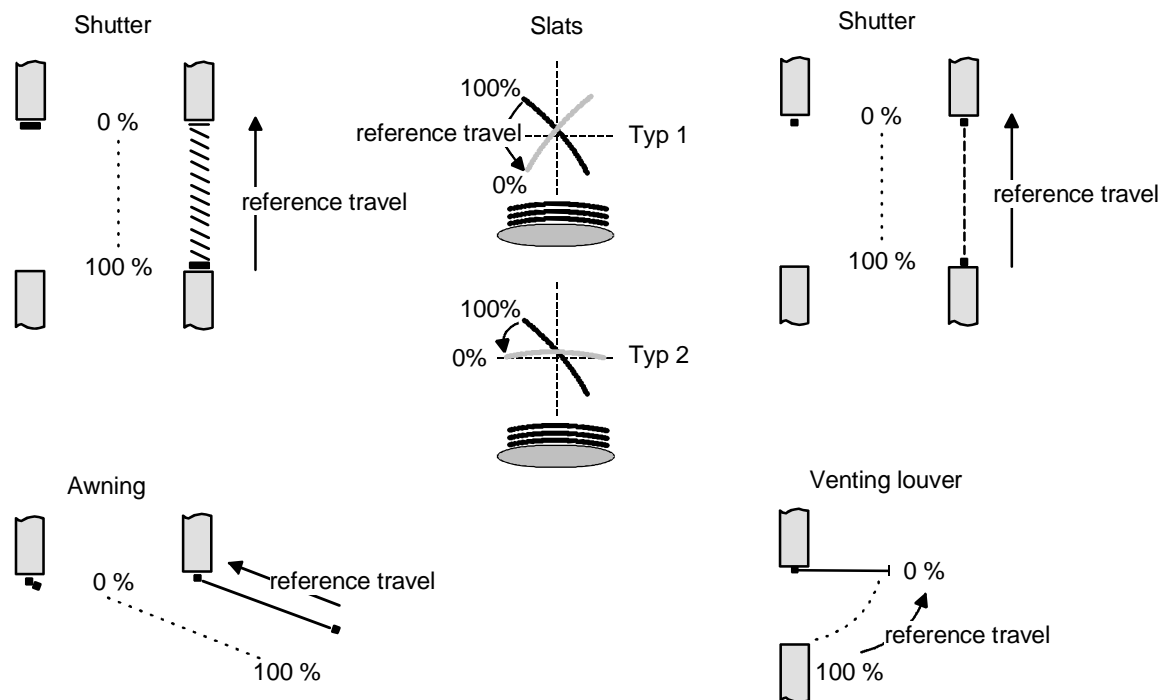
Fig. 29: Reference travel
