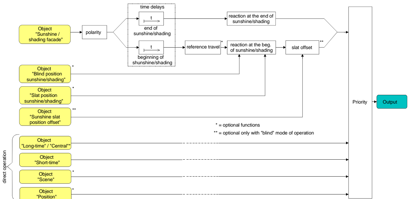
Fig. 33: Function diagram illustrating the sun protection
