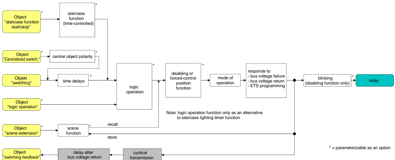
Fig. 12: Functional feedback diagram
